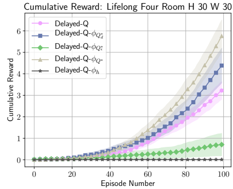
Figure 4: Delayed Q -Learning on a 30 \times 30 Four Rooms task distribution without the extraneous irrelevant feature of color and the paint action.
