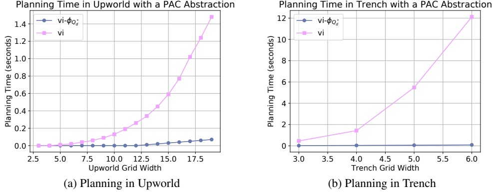
Figure 5: Planning time for Value Iteration with and without a state abstraction as the environmental state space grows. In all cases, the value of the computed policy is identical.
