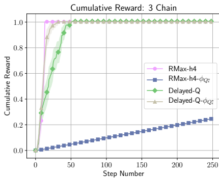
Figure 2: Results averaged over 50 runs on the pathological 3 chain MDP introduced in the proof of Theorem 3.5.
