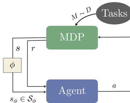
Figure 1: We study which state abstraction functions ( \phi ) are useful for lifelong RL, wherein the agent must learn to solve related tasks from the same distribution.
