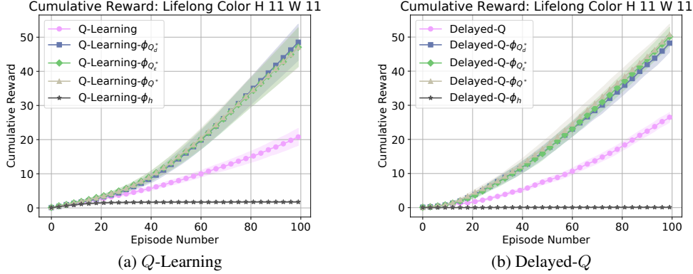
Figure 3: Cumulative reward averaged over 100 task samples from the Colored Four Rooms task distribution. Learning algorithms were given 100 episodes of 250 steps to learn, paired with a variety of different state-abstraction types.
