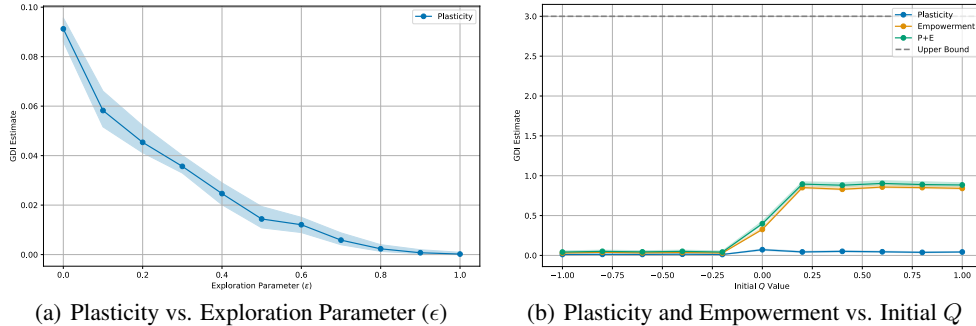
Figure 4: Results from two simple experiments that estimate plasticity, empowerment, and their sum with Q -learning ( Watkins and Dayan, 1992 ). On the left, we show the mean estimate of an \epsilon -greedy variant of Q -learning as a function of \epsilon , varied from zero to one, with bootstrapped confidence intervals. On the right, we show the estimate of plasticity (blue), empowerment (orange), and their sum (green), along with the upper bound (grey-dashed line) as a function of the initial Q value used by Q -learning, ranging from negative one to one. When Q = -1 , the agent is pessimistic, and when Q = 1 , the agent is optimistic.
